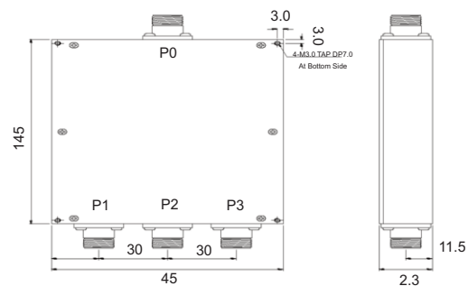
3 Way Power Divider
