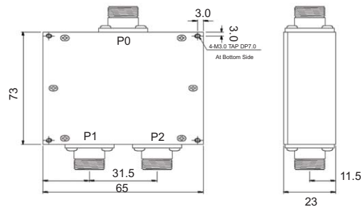
2 Way Power Divider
