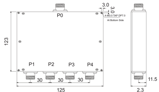
4 Way Power Divider
