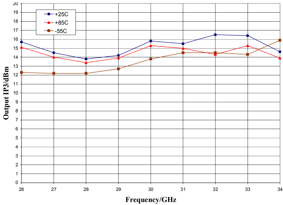
Output IP3 vs. Temperature, V_{dd} = 2.0\text{ V} , V_{gg} = 2.0\text{ V}
