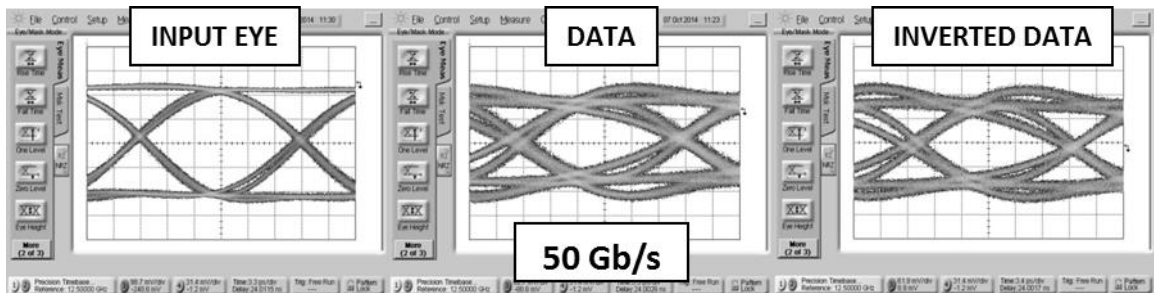
Oscilloscope measurements of the BAL-0067 with a 50 Gb/s PRBS pattern in single ended-to-differential mode. Eye diagrams are taken with a 2^{31}-1 PRBS input demonstrating minimal eye distortion/closure afforded by the extremely low frequency operation of the balun (<300 kHz).
